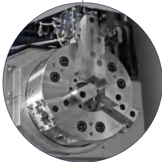
MAZAK | INTEGRIX I-250H S MAXIMUM MACHINING DIAMETER: Ø670 MM
