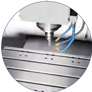
TSUGAMI | CNC MACHING CENTER X.Y.Z AXIS TRAVEL: 720×510×460MM | VA4
