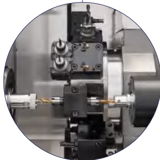
TSUGAMI | CNC PRECISION AUTOMATIC LATHE Ø3-Ø20 | S205A
